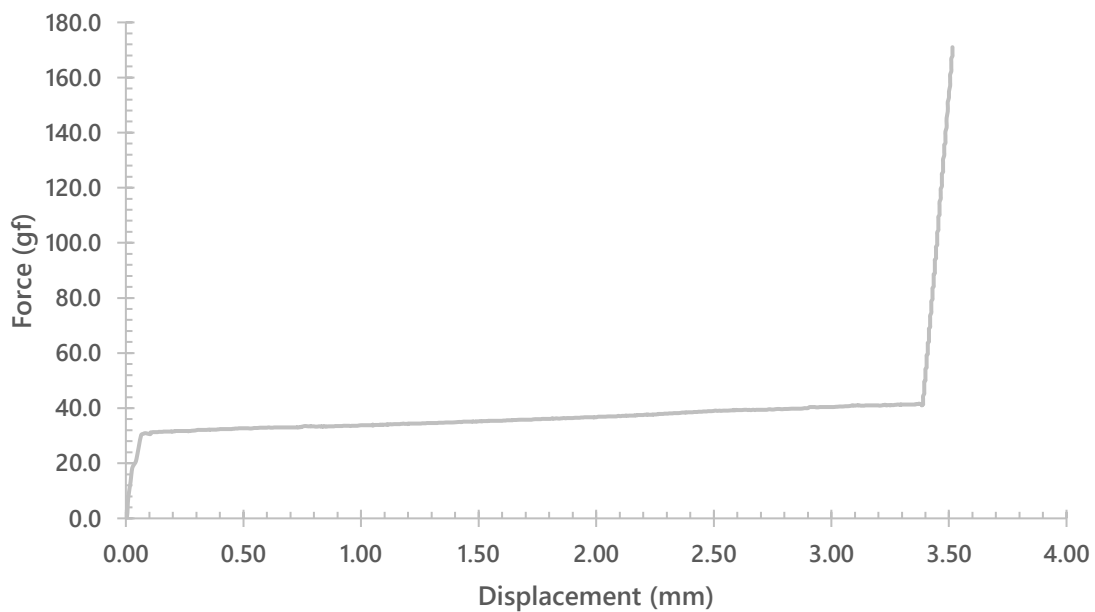
Gateron Magnetic Jade Delta Pink (Upstroke)
